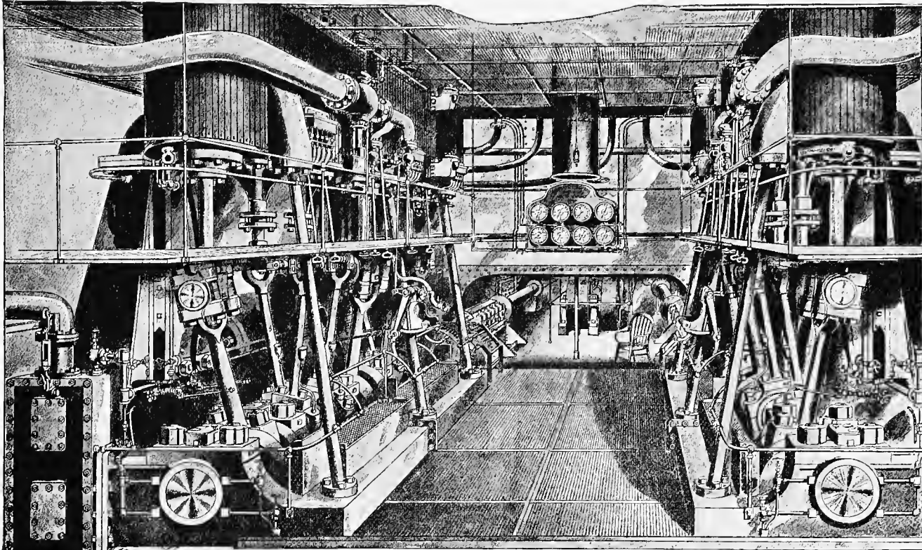
ENGINES OF TWIN-SCREW STEAMER RICHARD PECK.—Built by the Harlan & Hollingsworth Co., Wilmington, Del.
